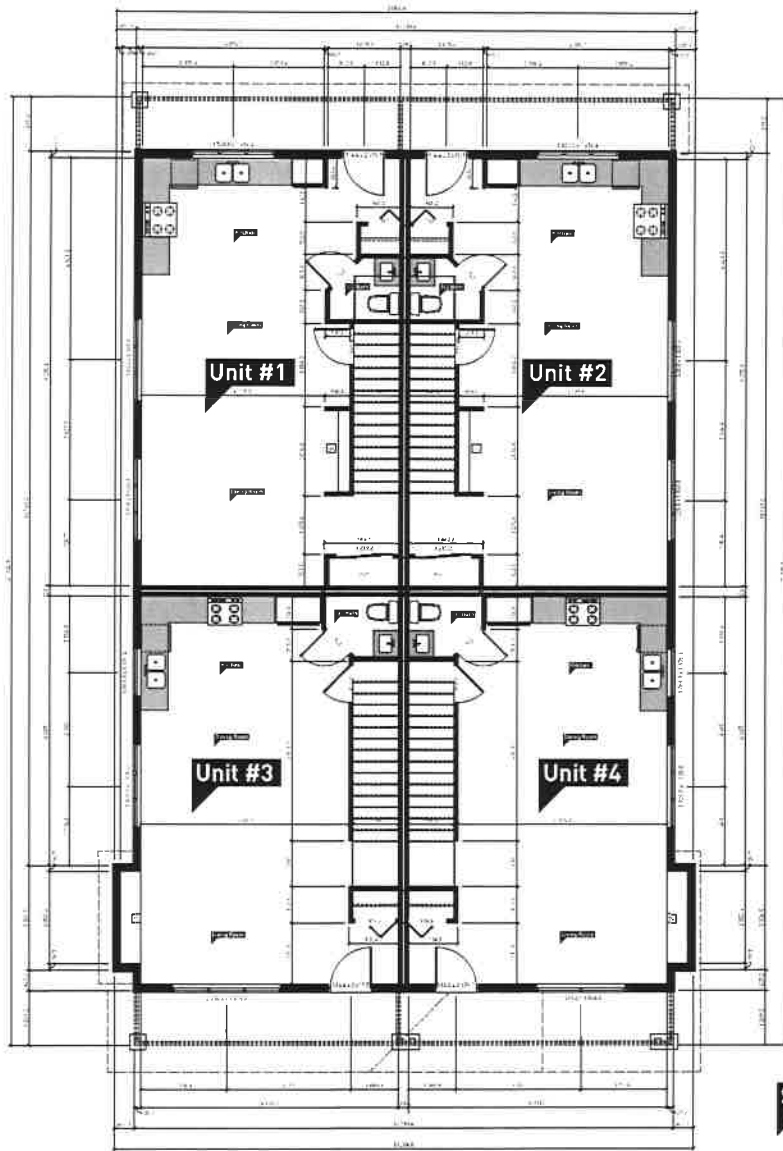
Main Floor Plan Scale: 1/32 Date: 2/28/17
